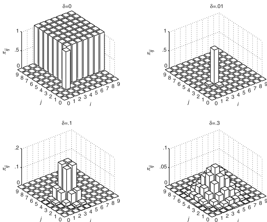
FIGURE 5 LIMITING DISTRIBUTION: QUANTITY COMPETITION
